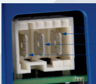
Fan power supply connector LUMBERG 3642-03
